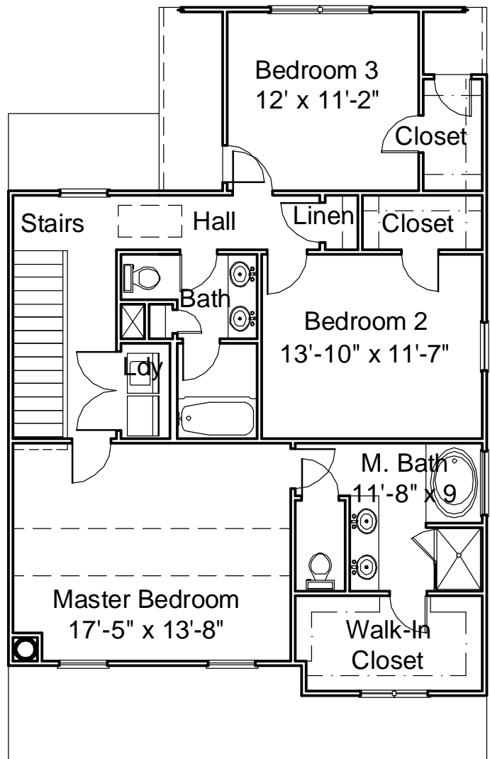
Second Floor
