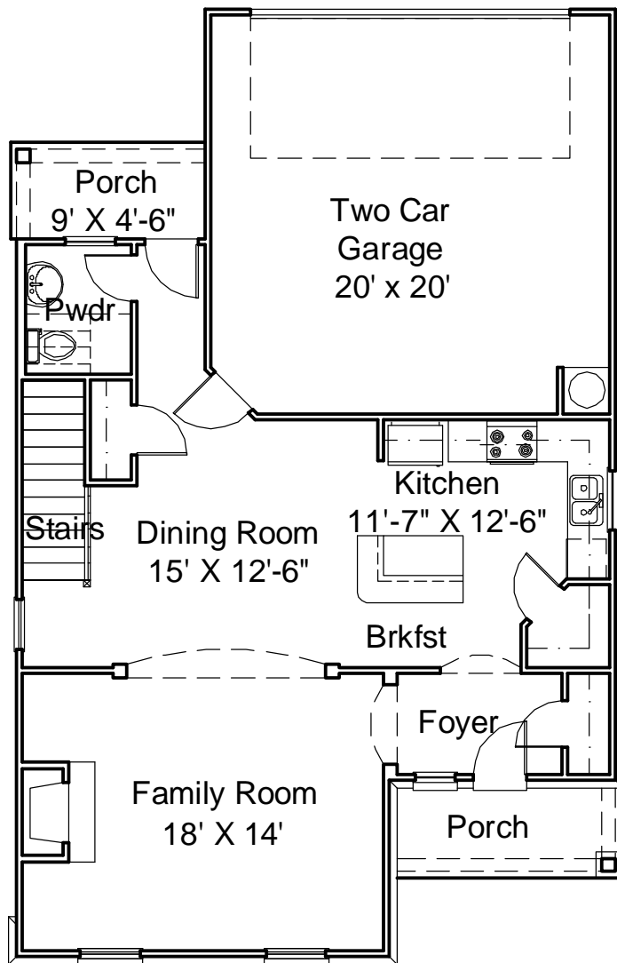
First Floor
