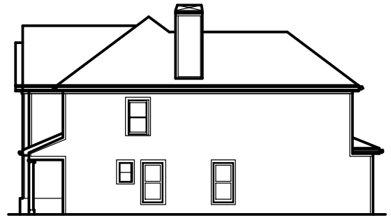
Left Elevation
