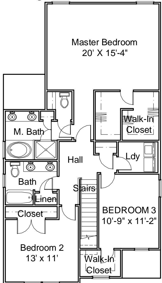
Second Floor
